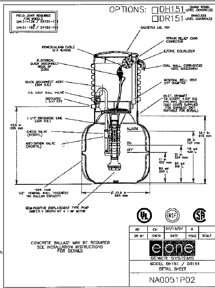
3 E/ONE DH151 GRINDER PUMP STATION
