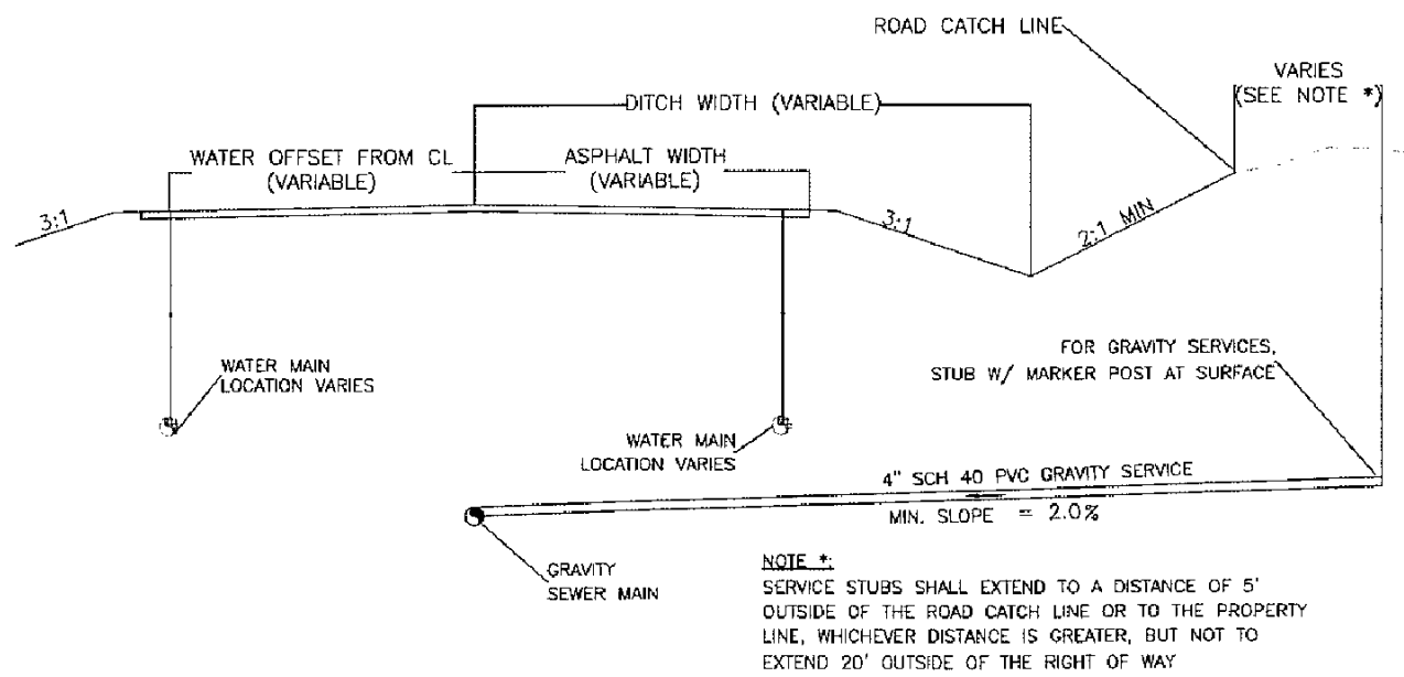
2 GRAVITY SEWER SERVICE DETAIL
