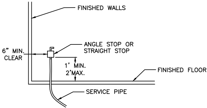
1" HDPE SERVICES PROFILE VIEW
