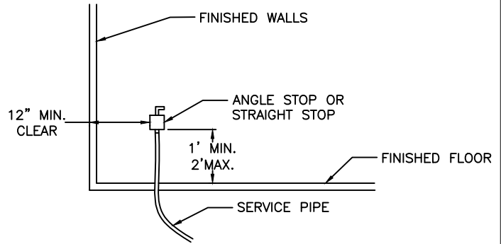
1 1/2" AND 2" HDPE SERVICES PROFILE VIEW
