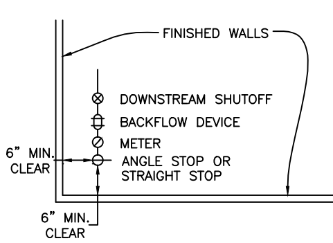
1" HDPE SERVICES PROFILE VIEW
