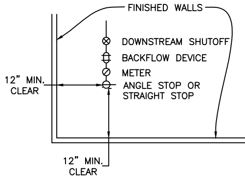
1 1/2" AND 2" HDPE SERVICES PROFILE VIEW
